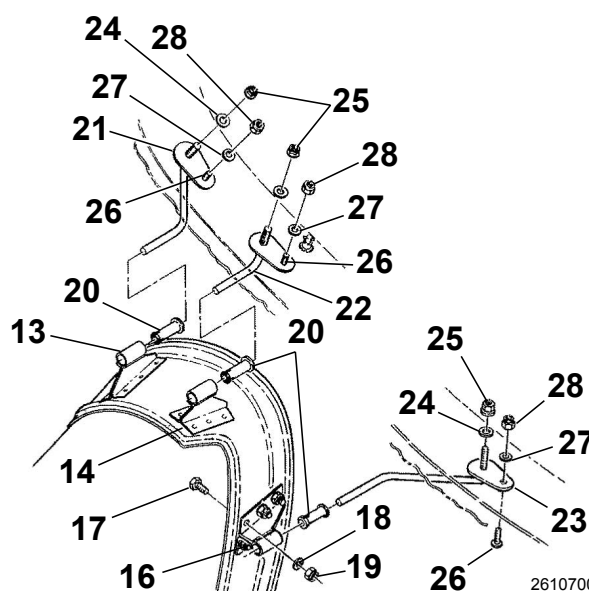
ENGINE EXHAUST DUCT INSTALLATION - 208 -0001 & ON AND 208B -B0001 THRU B-1990 WITH CARGO POD AND 208B -B5000 & ON WITH OR WITHOUT CARGO POD Figure 04. (Sheet 1)
