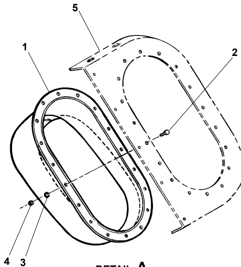
PRIMARY EXHAUST DUCT INSTALLATION Figure 01. (Sheet 1)
