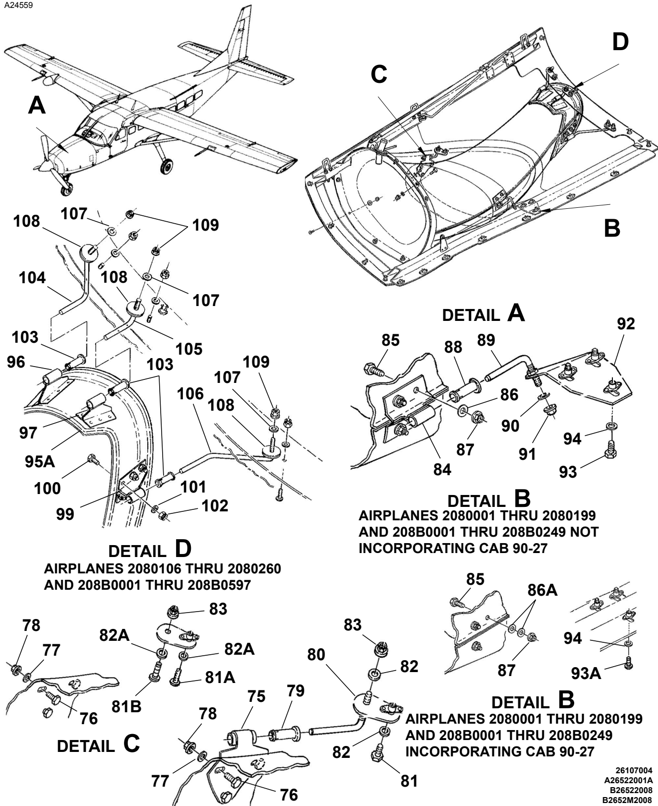
ENGINE EXHAUST DUCT INSTALLATION - 208-B0001 & ON AND 208B-B0001 THRU -B4999 WITH CARGO POD AND 208B-B5000 & ON WITH OR WITHOUT CARGO POD Figure 04. (Sheet 2)
