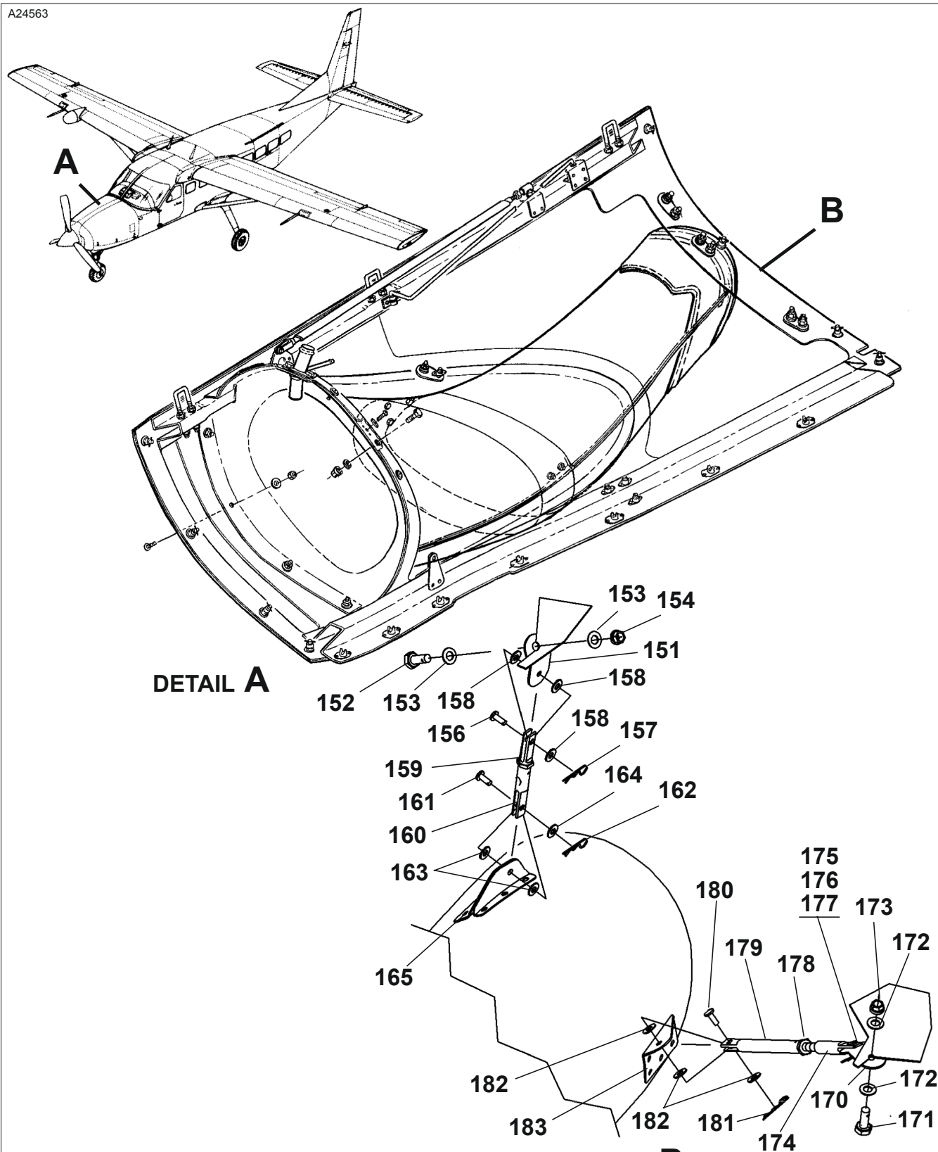
ENGINE EXHAUST DUCT INSTALLATION - 208 -0001 & ON AND 208B -B0001 THRU -B4999 WITH CARGO POD AND 208B -B5000 & ON WITH OR WITHOUT CARGO POD
